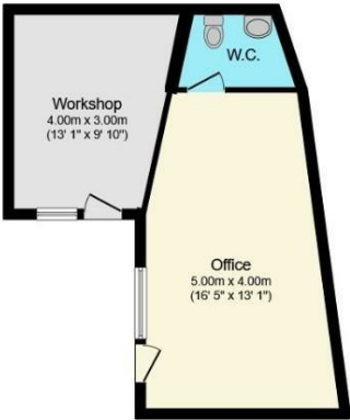
Outbuilding Floor area 38.5 sq.m. (414 sq.ft.)
